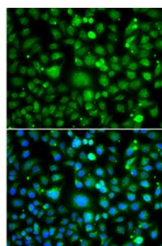
Fig. 2. Immunofluorescence analysis of MCF-7 cells using TEK antibody. Blue: DAPI for nuclear staining.
